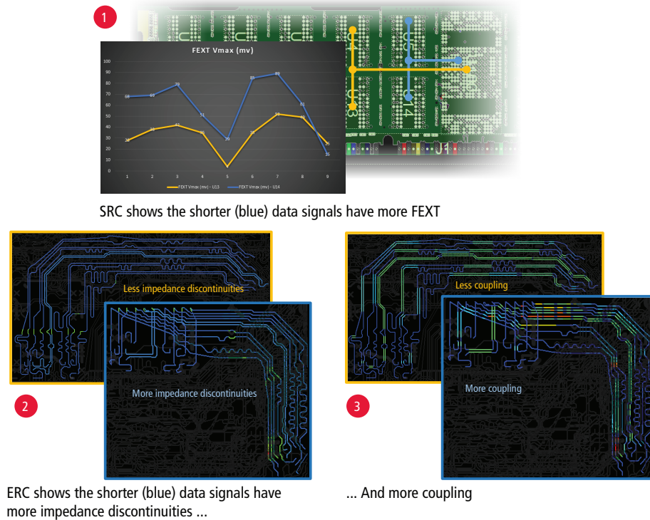
Figure 3: SRC/ERC example
