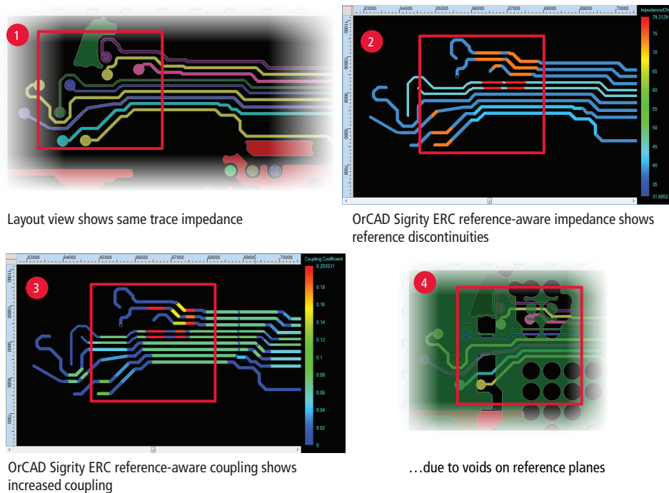
Figure 1: OrCAD Sigrity ERC reference-aware impedance/coupling overlay
